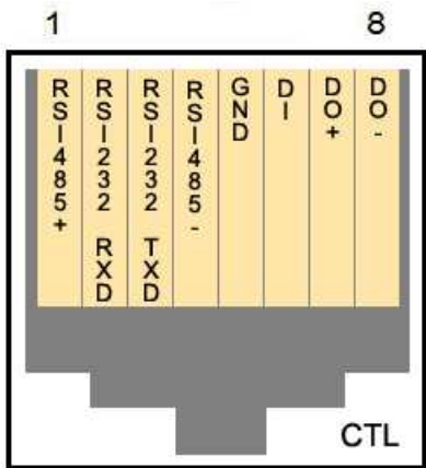
Picture 4 : CTL Port Description
